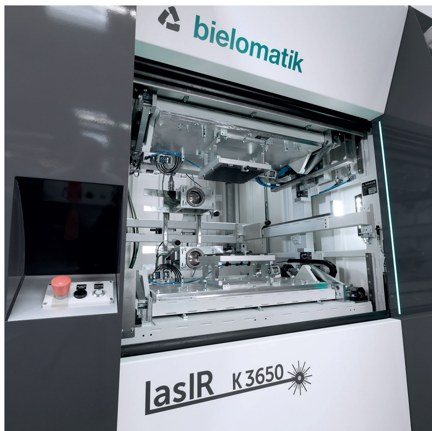
Turn2Weld technique: the newly developed welding machine uses one laser per part and swivels the machine tables through 90° toward the laser scanners with the aid of servo motors (© bielomatik)
